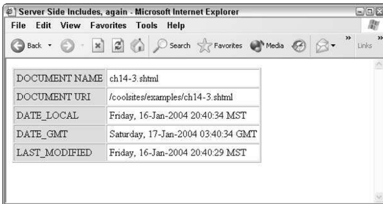
Figure 14-3: You can use SSI variables to display interesting information.
