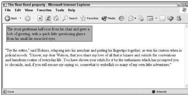
Figure 12-11: Relative positioning makes the container part of the regular document flow.
