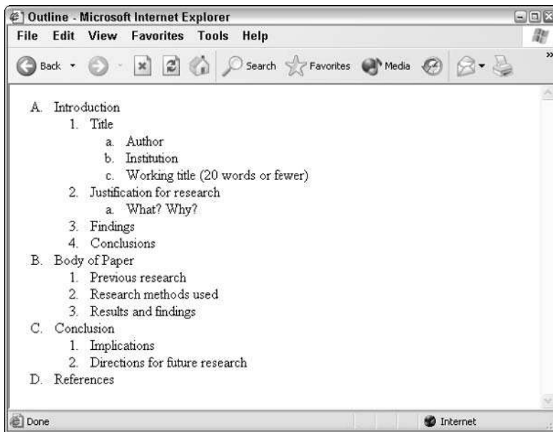
Figure 5-7: An outline using special <ol> attributes to display varied types of numbers and letters.
