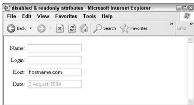
Figure 10-7: The disabled and readonly attributes rendered in Internet Explorer.
