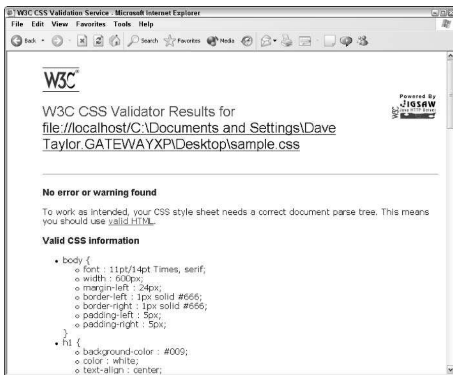
Figure 16-7: CSS document validates!
