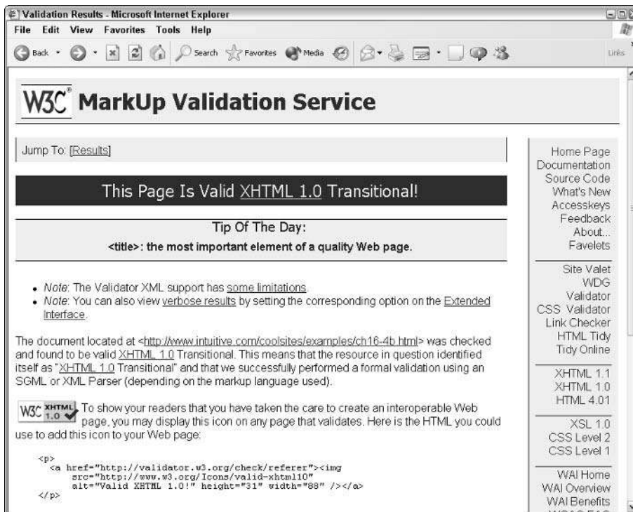
Figure 16-4: A few simple changes result in valid XHTML 1.0 transitional code.
