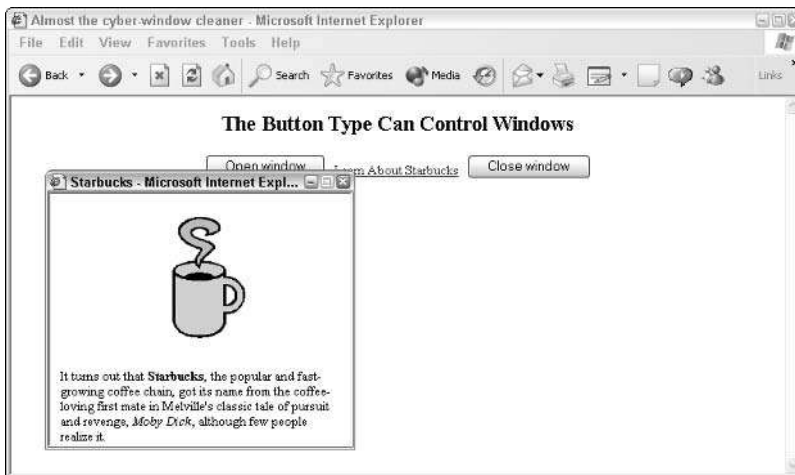
Figure 10-2: Pop-up navigational controls implemented with JavaScript and an empty HTML form.
