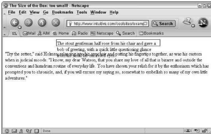
Figure 12-7: Don't specify a height that's too small to contain the text, or the text spills out of the container.
